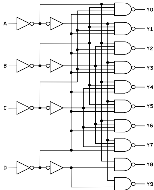
Figure 2. Logic diagrams – Continued.
