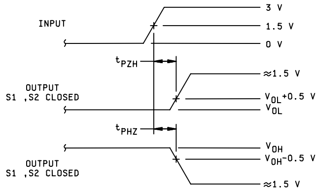
Waveform for t_{PLZ} and t_{PHZ}
