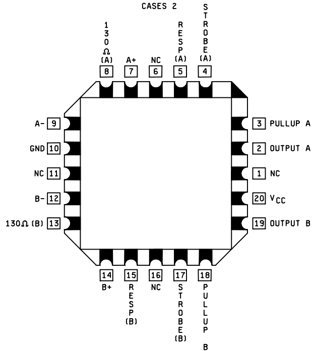
Figure 1. Logic diagrams and terminal connections – Continued.
