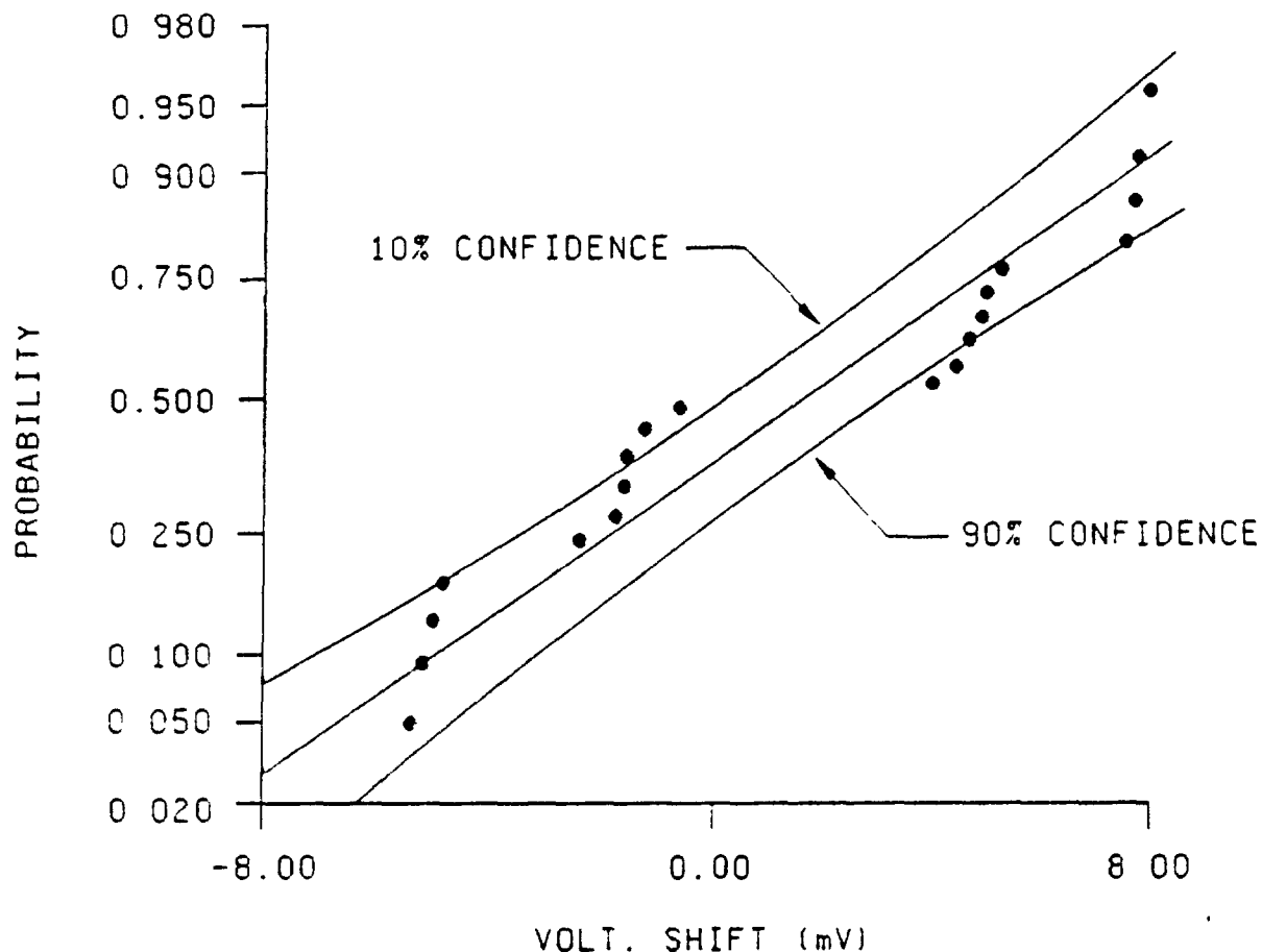
FIGURE 11 Normal probability plot of actual data that exhibited systematic effects
