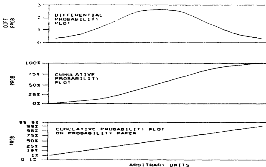
FIGURE 5 What is probability paper?
