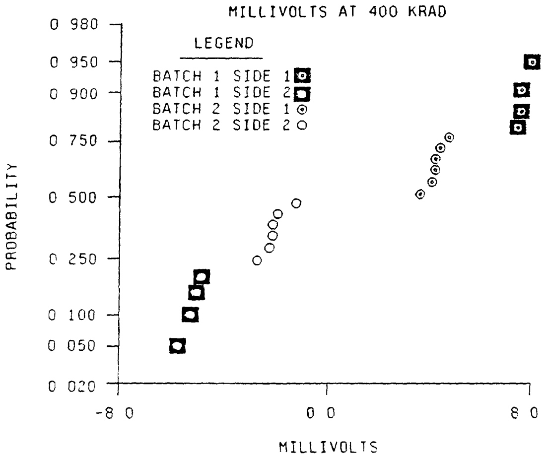
FIGURE 12 Plot of figure 11 with confidence lines omitted and points "colored"
