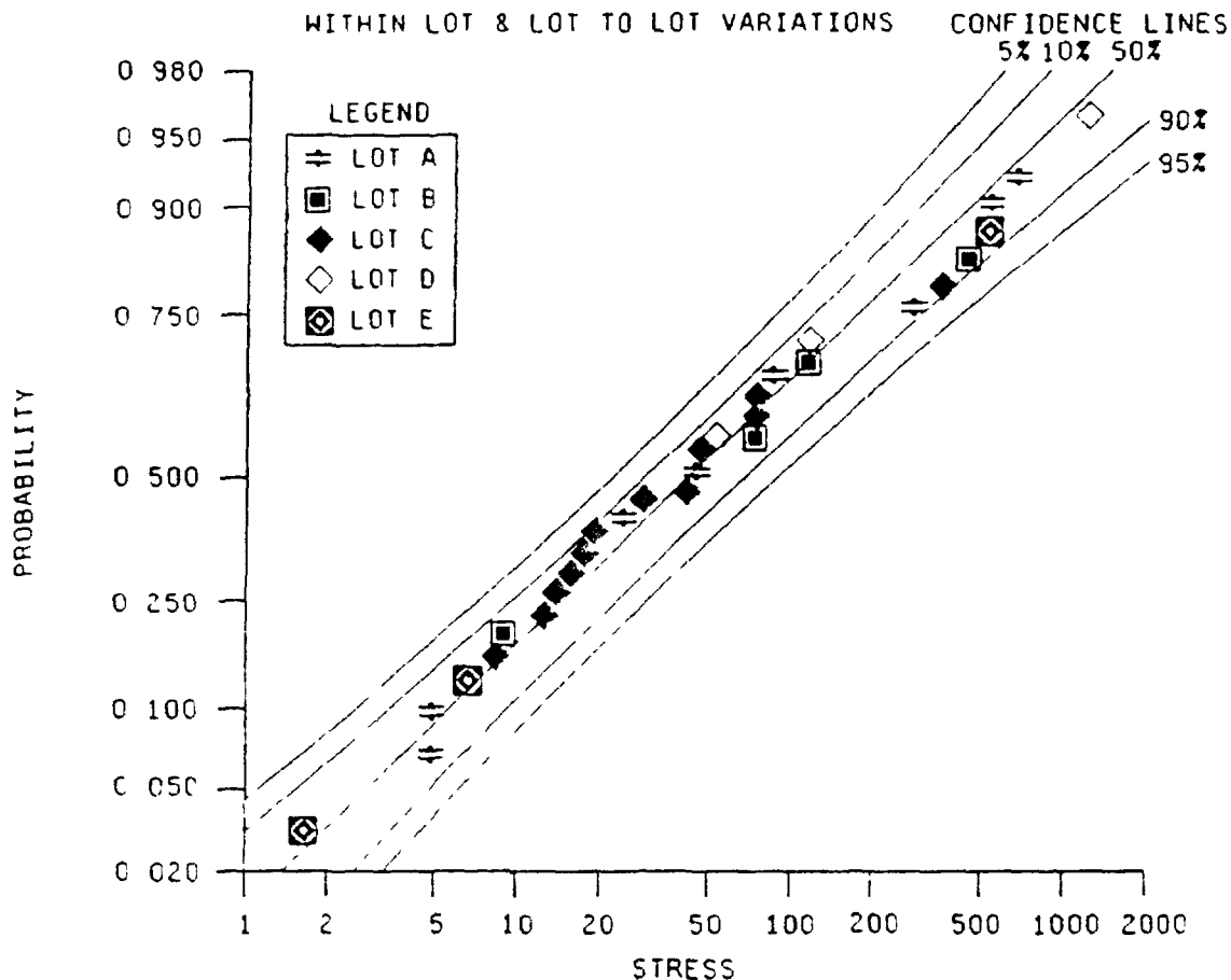
FIGURE 14 Within-lot variations exceed lot-to-lot variations
