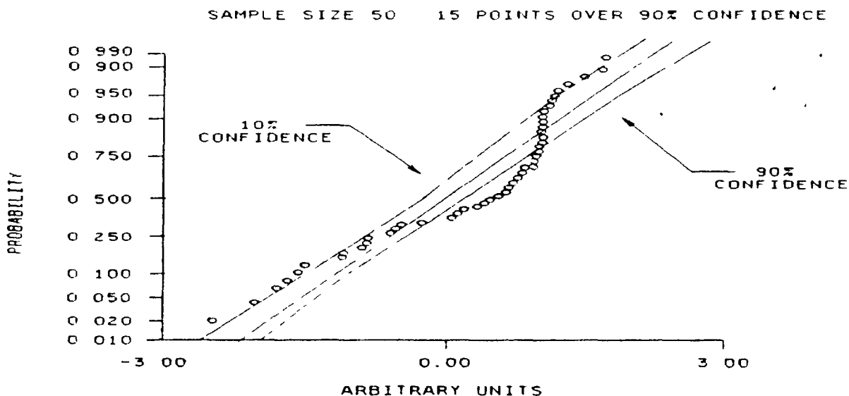
FIGURE 9 Normal probability plot of 50 points with an overly good but still acceptable -simulated data
