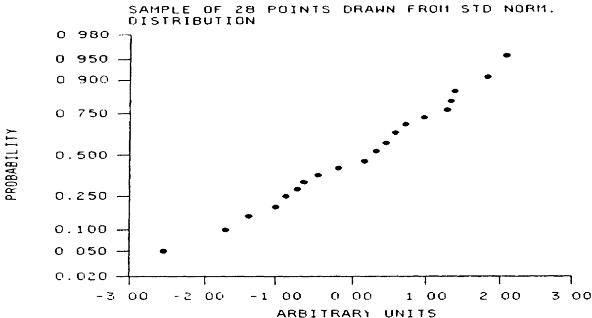
FIGURE 6 Sample normal probability plot of 20 points - simulated data
