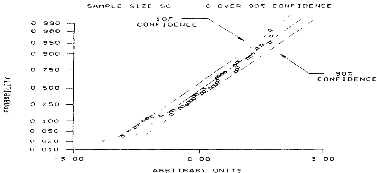
FIGURE 8 Ideal normal probability plot with 50 points -simulated data
