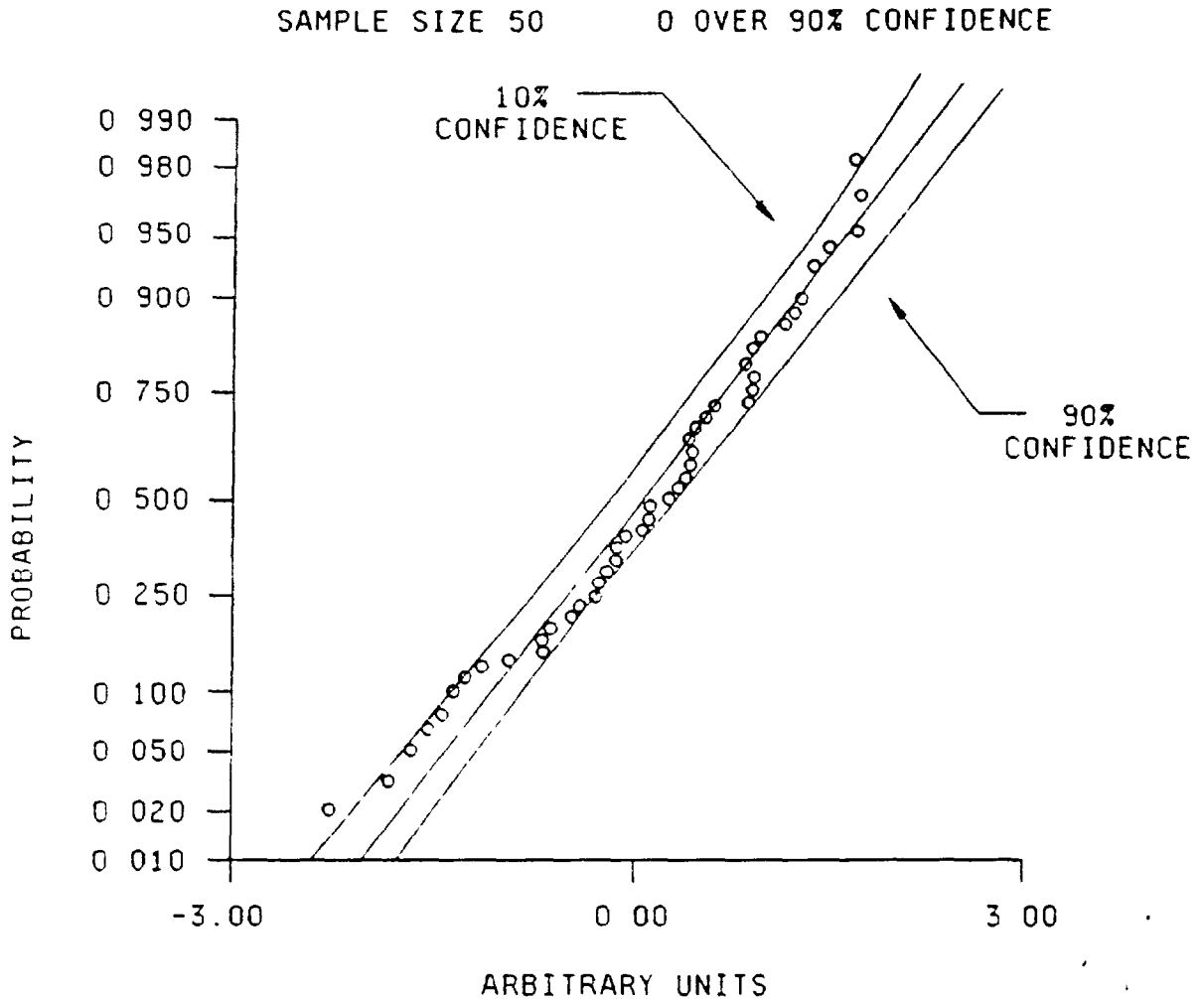
FIGURE 10 Normal probability plot of 50 points with an exceptionally bad fit -simulated data
