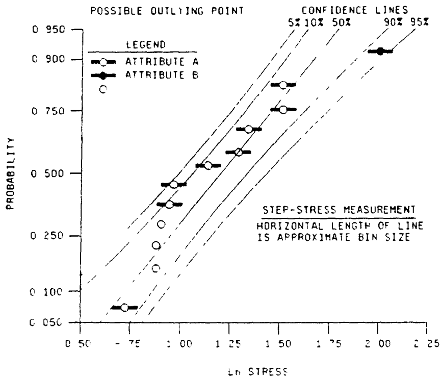
FIGURE 13 Double example of possible outlier and step-stress data - actual data
