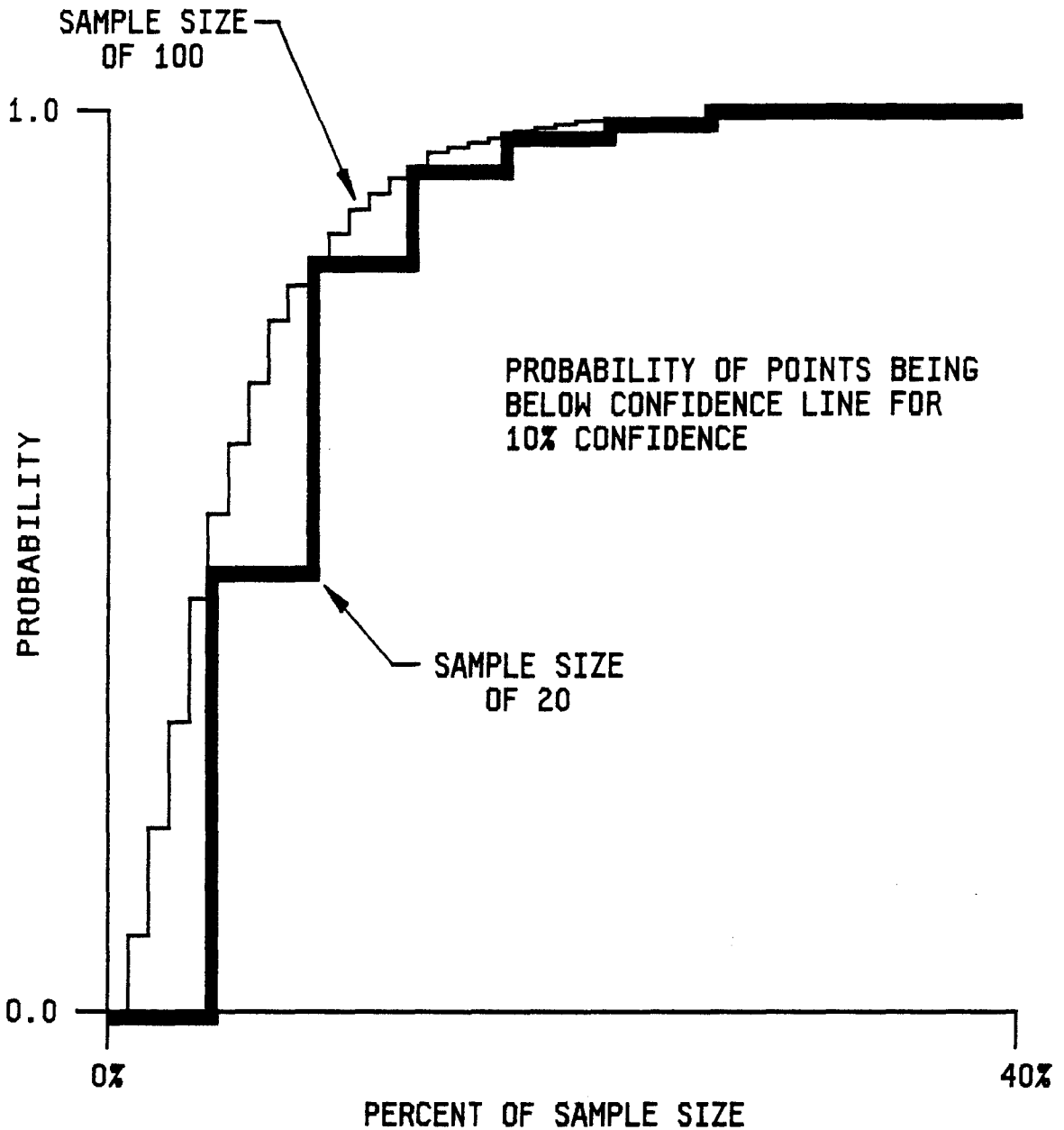
FIGURE 17. Expected fraction of devices which exceed 10 percent confidence line. Sample sizes of 20 and 100.
