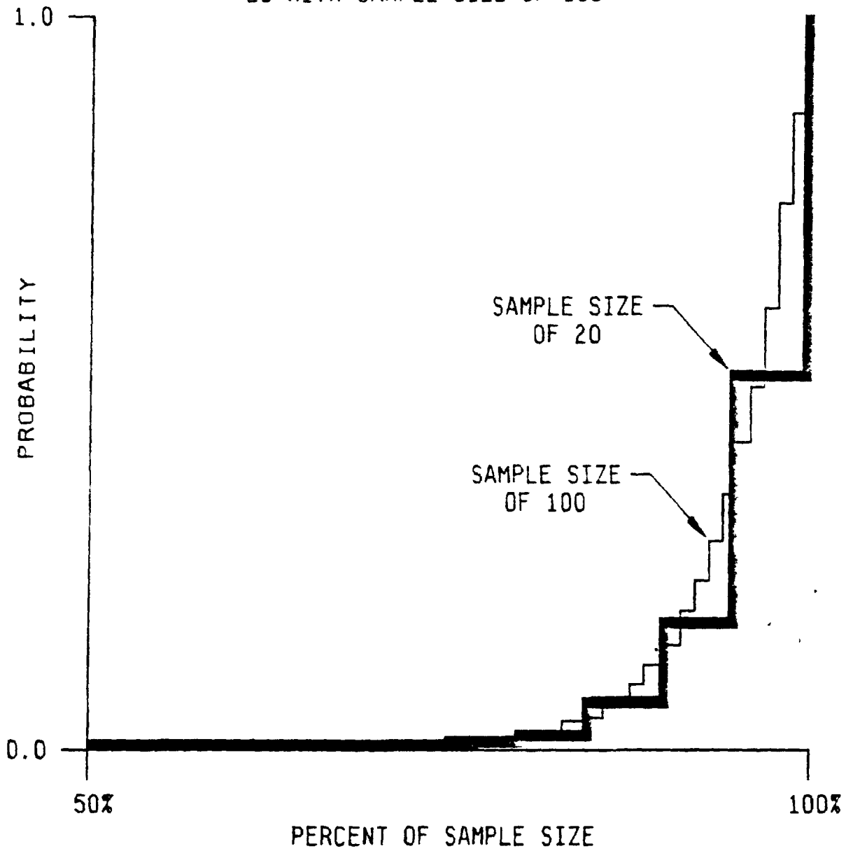
FIGURE 16 Expected fraction of devices which exceed 90 percent confidence line Sample sizes of 20 and 100
