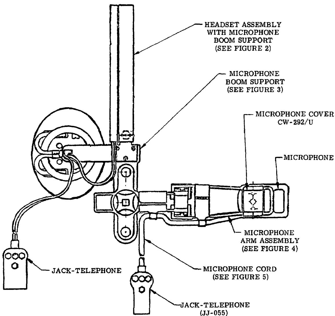
FIGURE 1. H-63( )/U Assembly.
