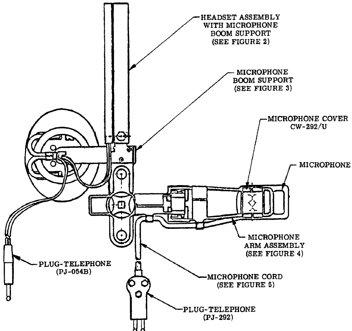
FIGURE 1. H-62( )/U Assembly.
