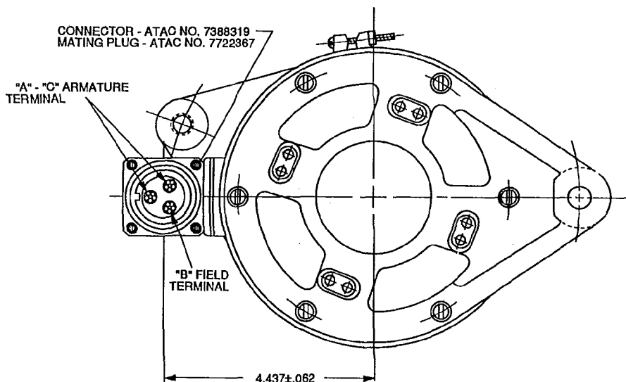
COMMUTATOR END VIEW
