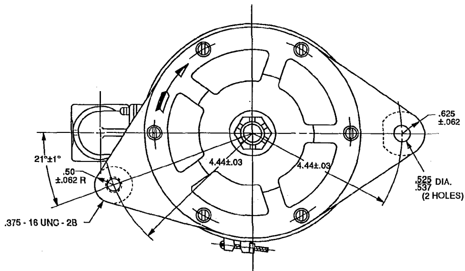
ROTATION C. W. DRIVE END VIEW
