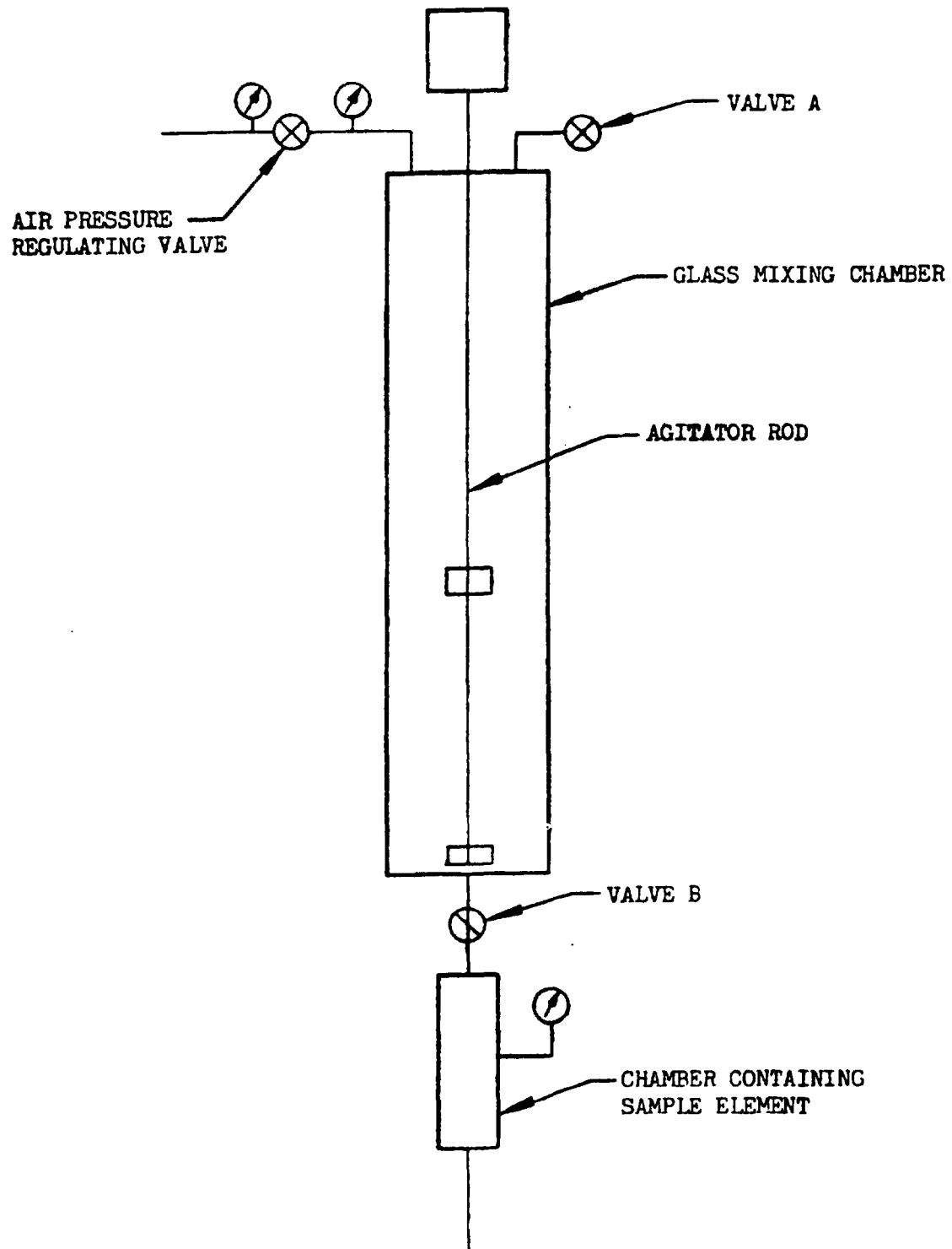
FIGURE 5. Apparatus for determining filtration efficiency of line-type elements.
