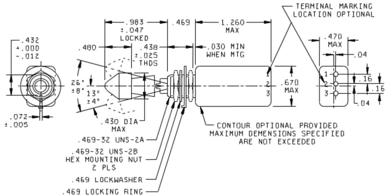
FIGURE 1. Dimensions and configuration - Continued.
