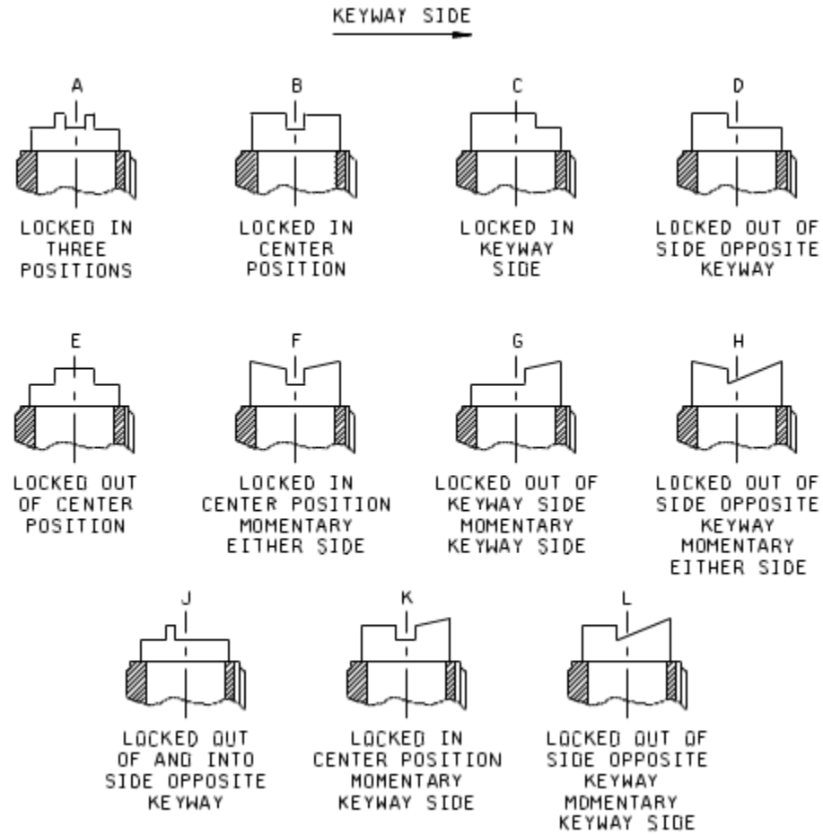
FIGURE 1. Dimensions and configuration - Continued.
