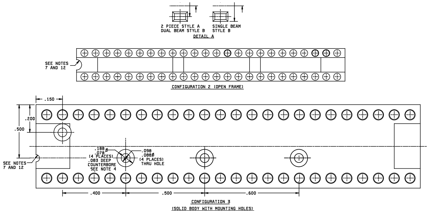
FIGURE 1. Dimensions and configurations - Continued.
