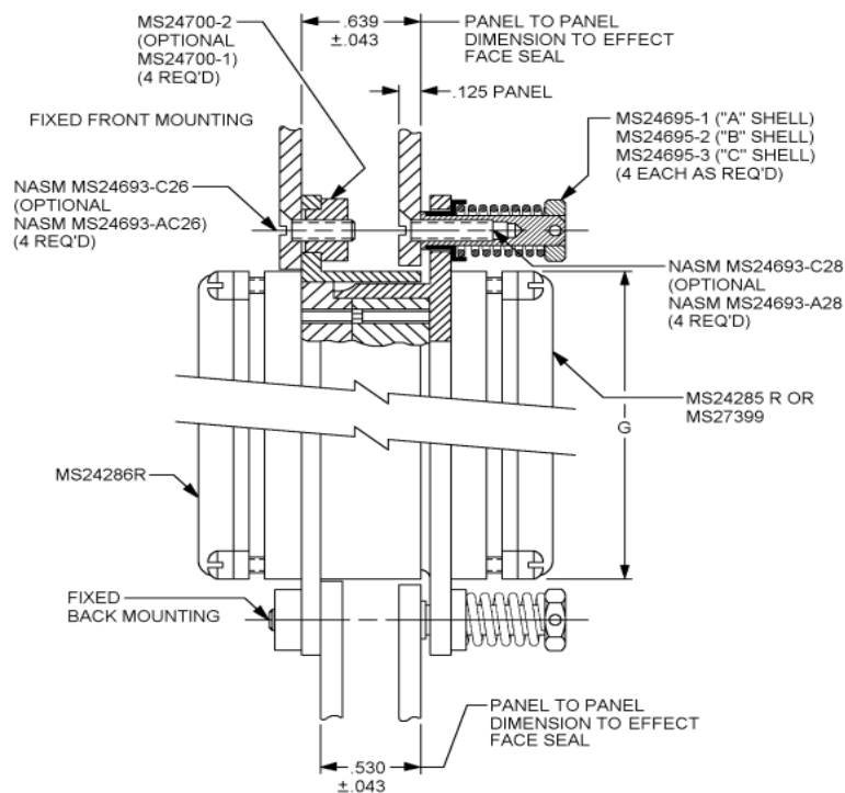
FIGURE 1. Connector mating and mounting details.
