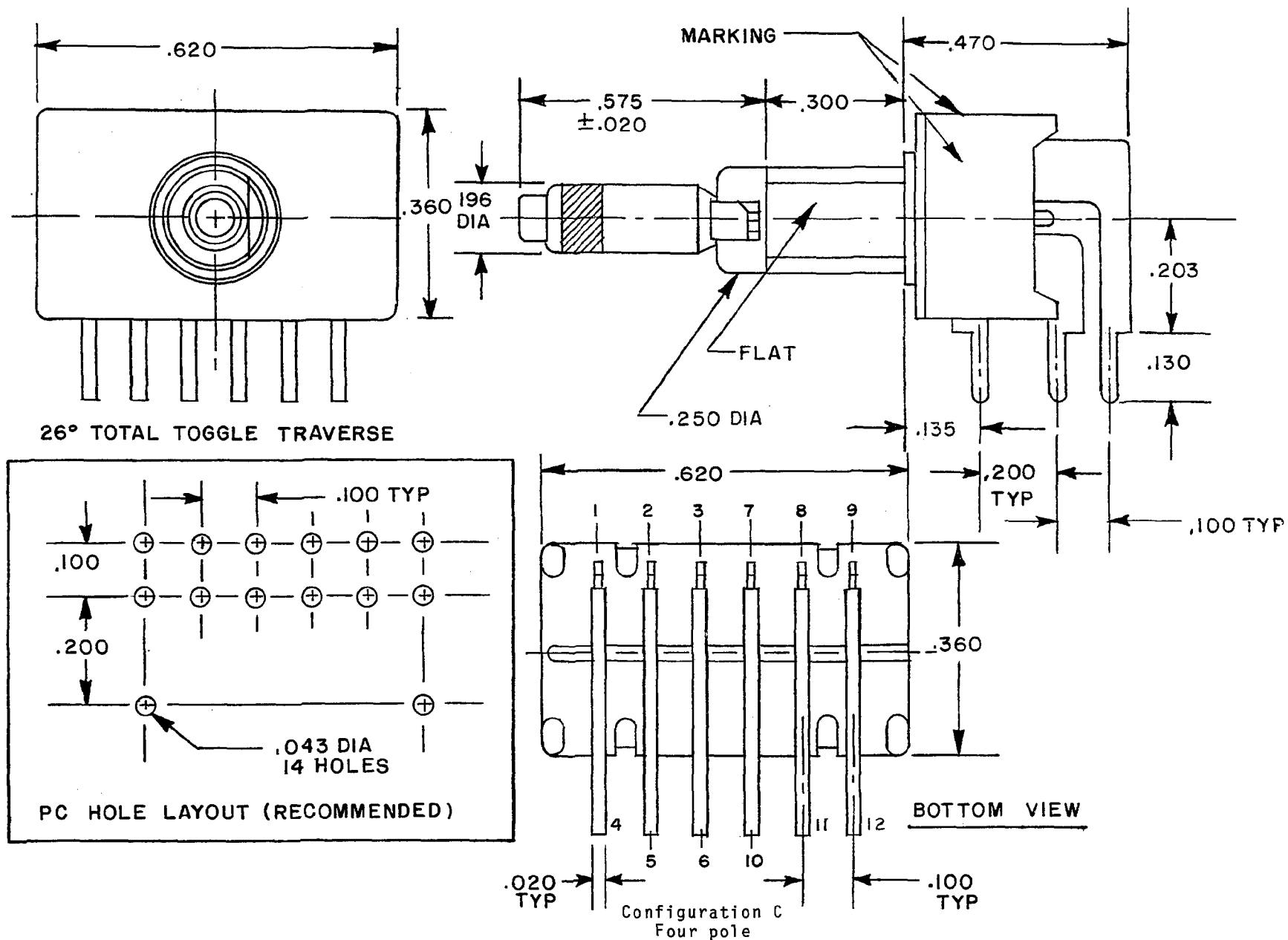
FIGURE 1. Dimensions and configurations - Continued.
