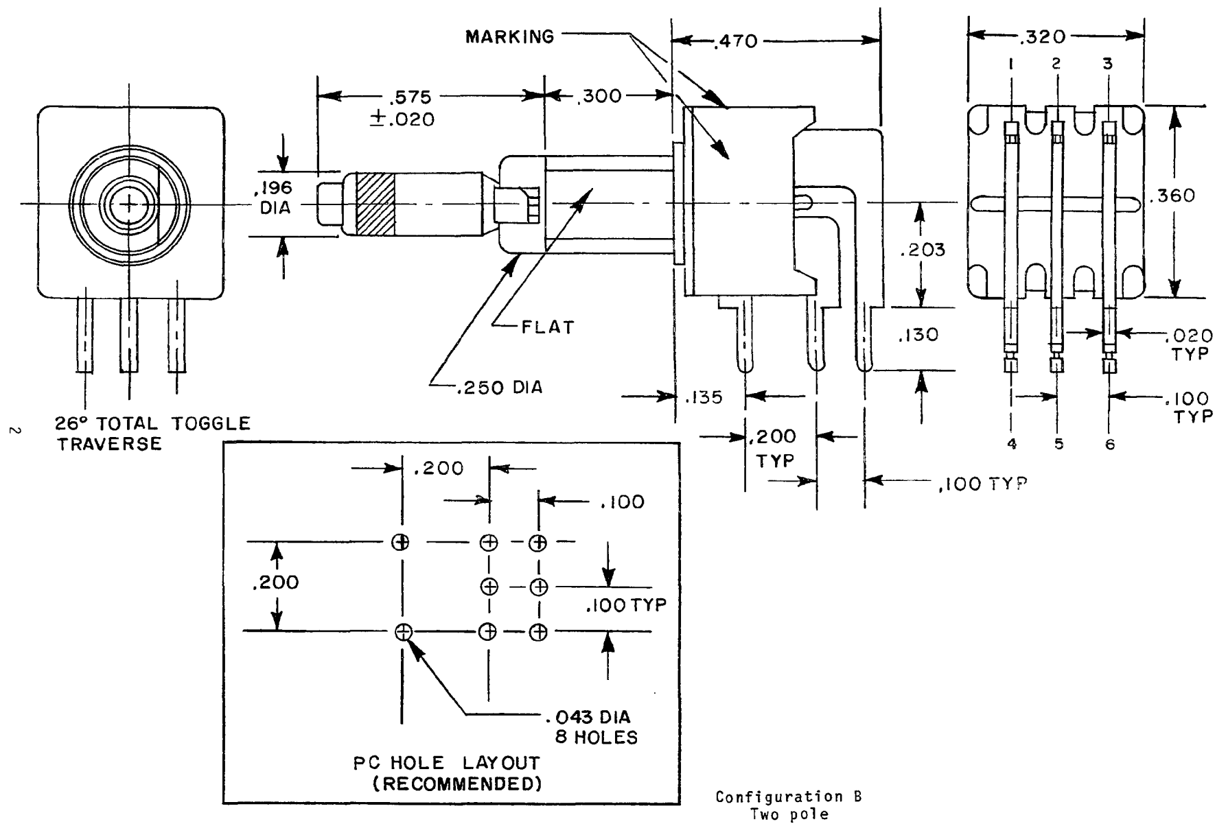
FIGURE 1. Dimensions and configurations - Continued.
