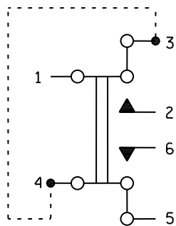
FIGURE 8. Wiring for 3-Way Switches (Function 4).
