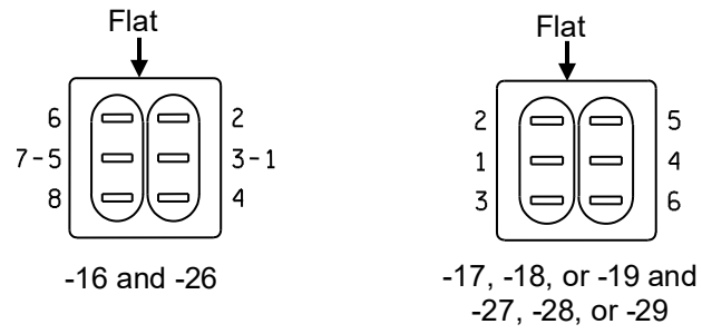
FIGURE 7. Terminal Identification
