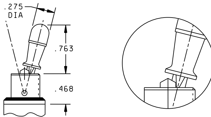
2 Locked Positions
