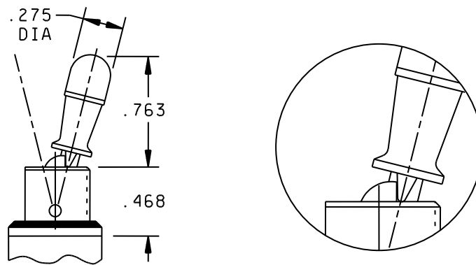
1 Locked Position
