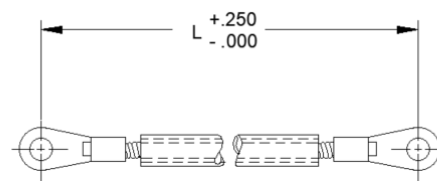
ASSEMBLY TYPES I, J, K, L
