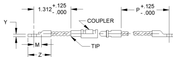
ASSEMBLY TYPE E SHORT END
