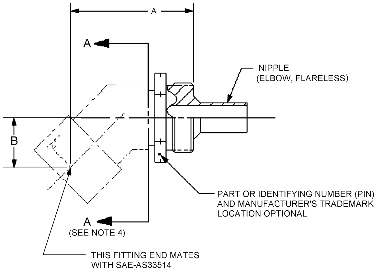
FIGURE 1. Flareless, 45°, elbow sub assembly.
