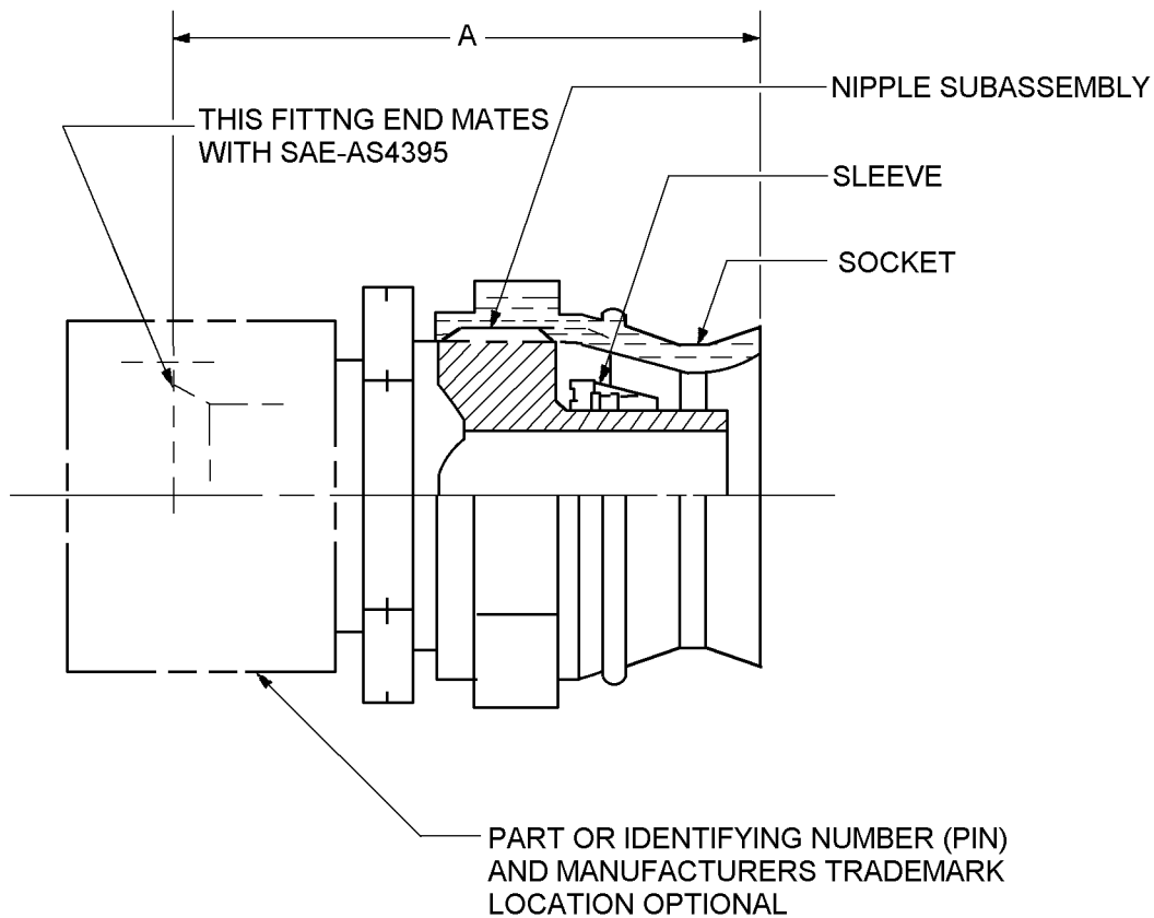
FIGURE 1. Straight, flared, adapter assembly.
