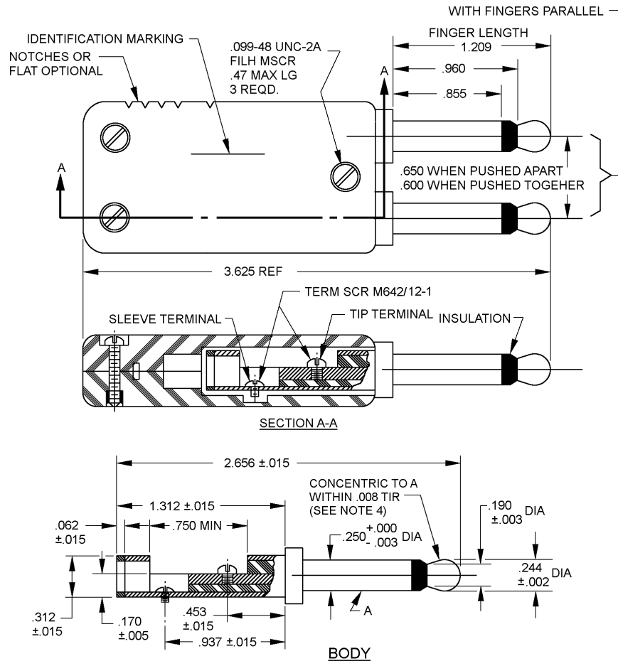
FIGURE 1. Dimensions and configuration.
