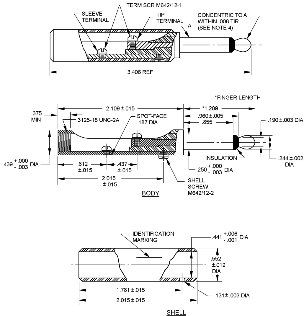
FIGURE 1. Dimensions and configuration.
