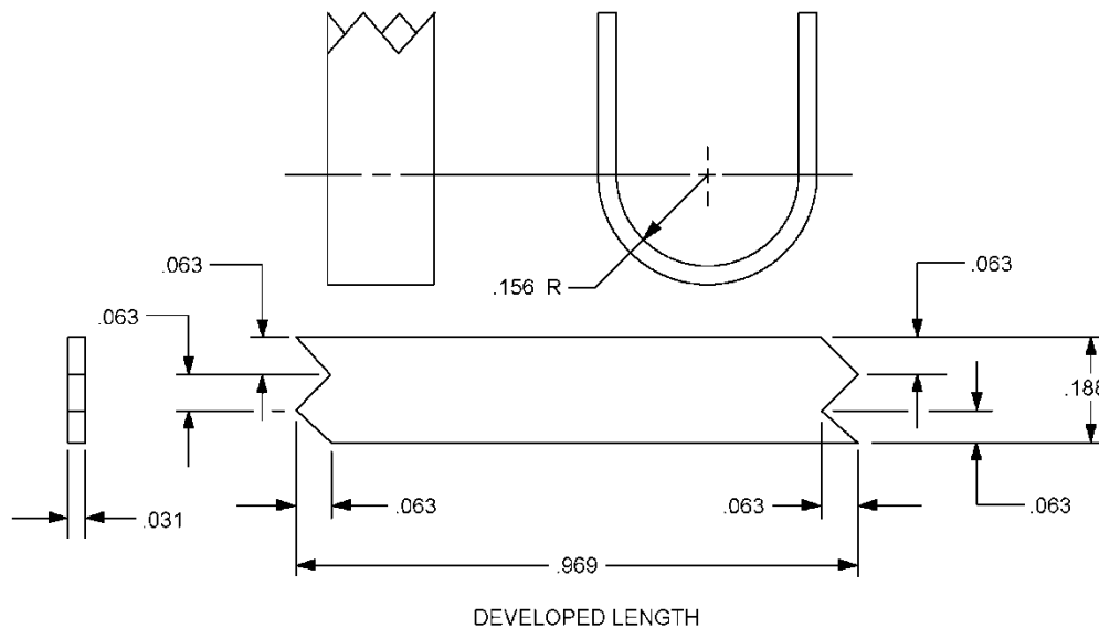
FIGURE 1. Dimensions and configuration - Continued.
