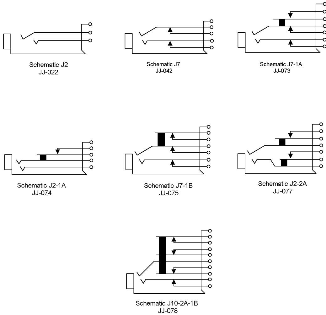
FIGURE 1. Dimensions and configuration - Continued.
