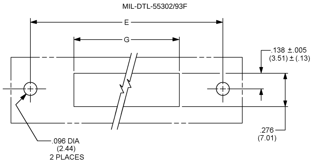
TYPICAL HOLE CUTOUT FOR CRIMPABLE CONTACT
