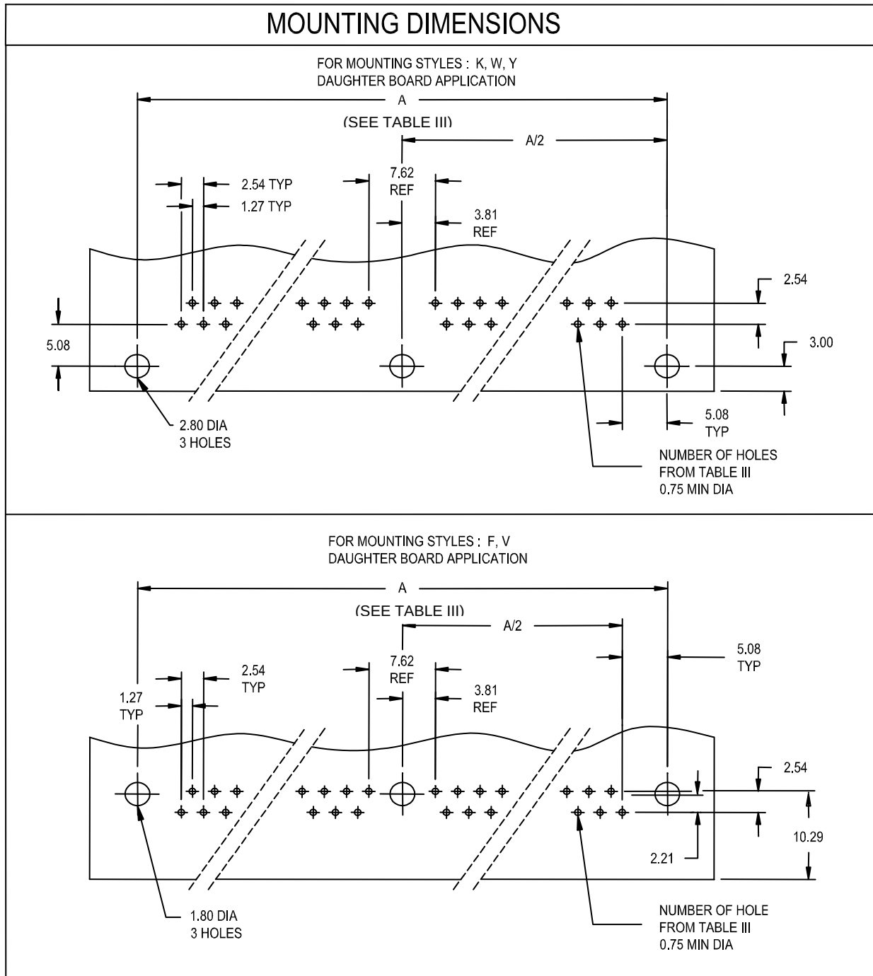
FIGURE 5. Mounting dimensions – Continued.
