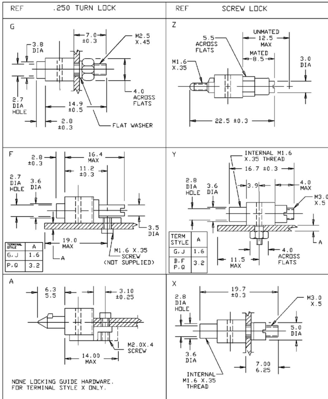
FIGURE 4. Locking hardware.
