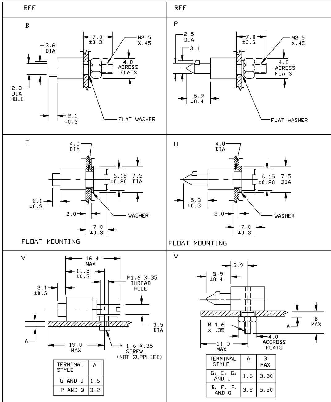
FIGURE 3. Mounting styles.
