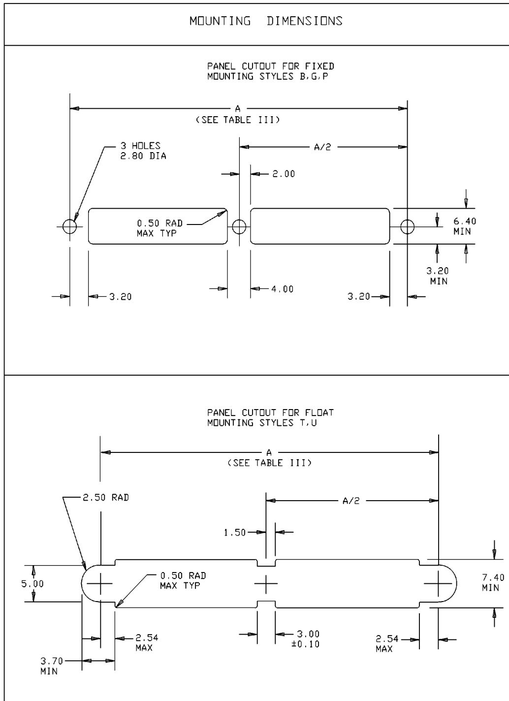
FIGURE 5. Mounting dimensions – Continued.
