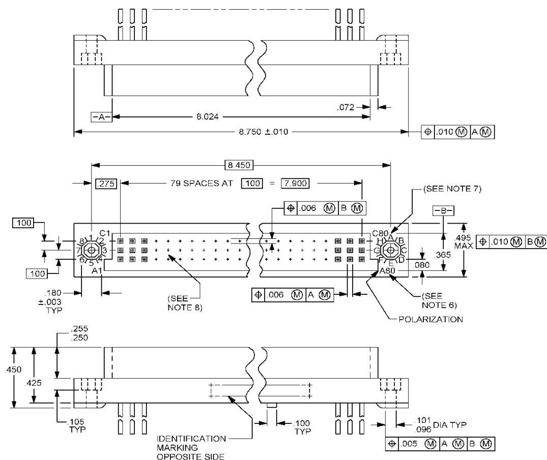
FIGURE 1. Connectors, kit receptacle, .100 (25.4 mm) spacing, 160 and 240 contacts.
