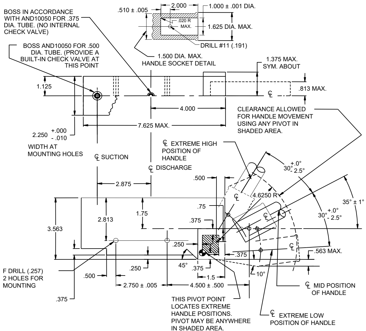
FIGURE 1. Hydraulic hand pump.
