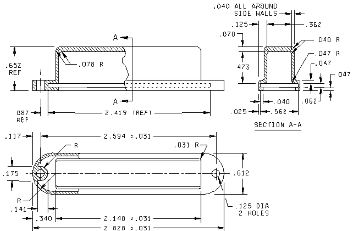
FIGURE 1. Dimensions and configuration.
