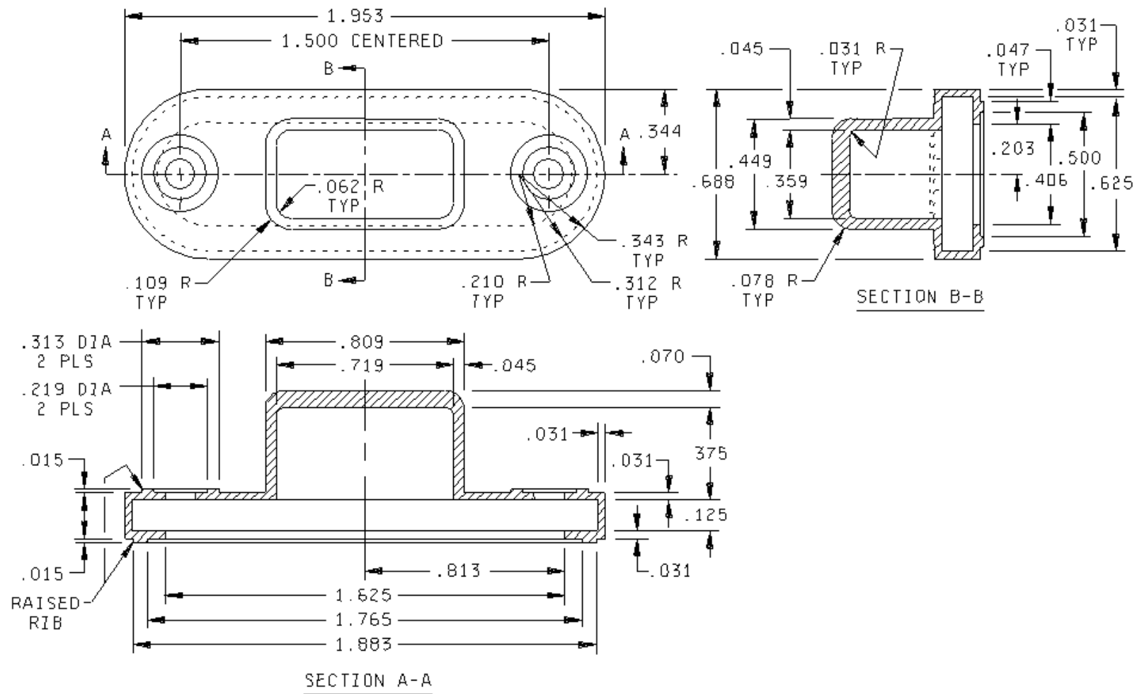
FIGURE 1. Dimensions and configuration – Continued.
