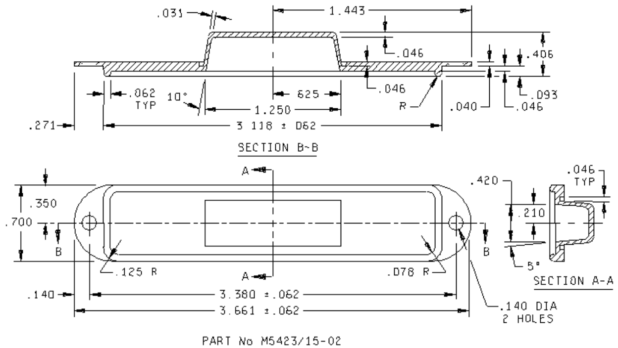
FIGURE 1. Dimensions and configuration – Continued.
