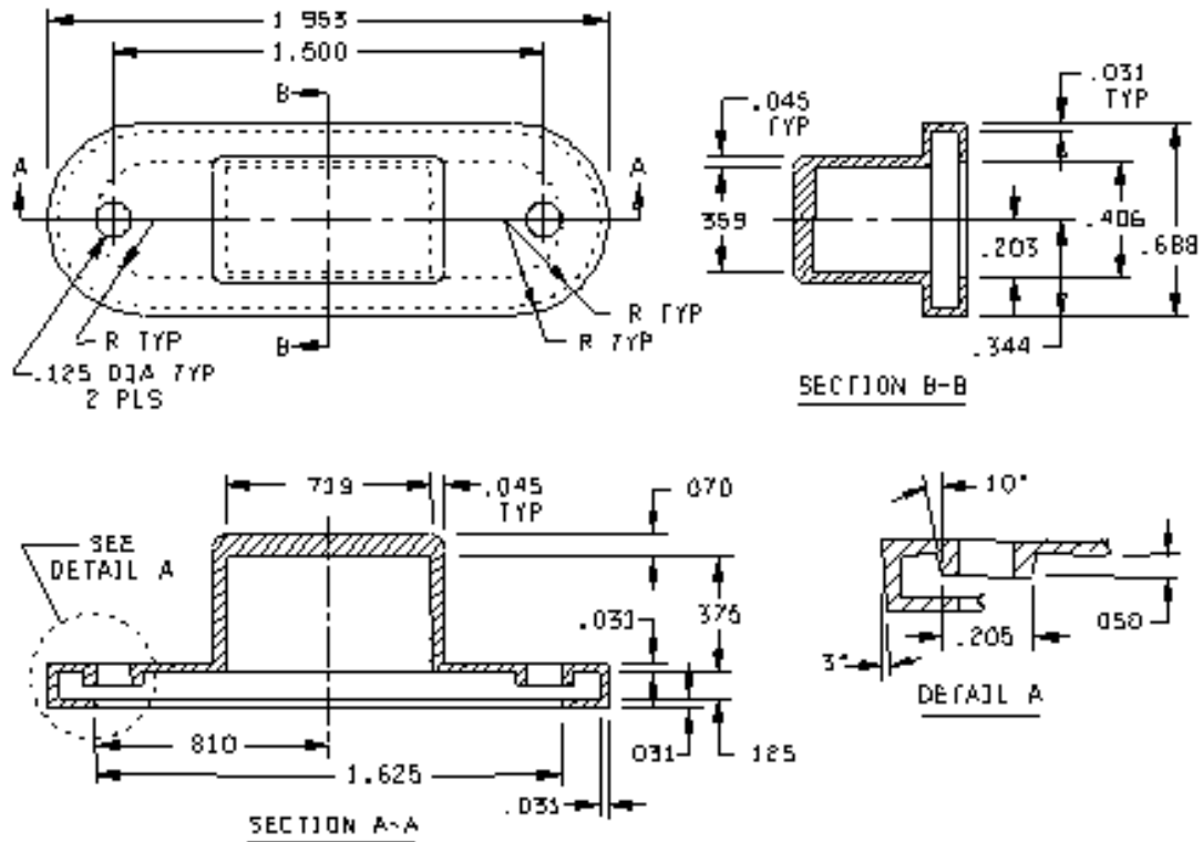
PART No M5423/15-03 ALTERNATE CONFIGURATION
