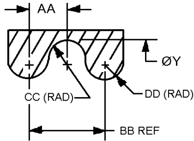
ENLARGED VIEW OF U THREAD
