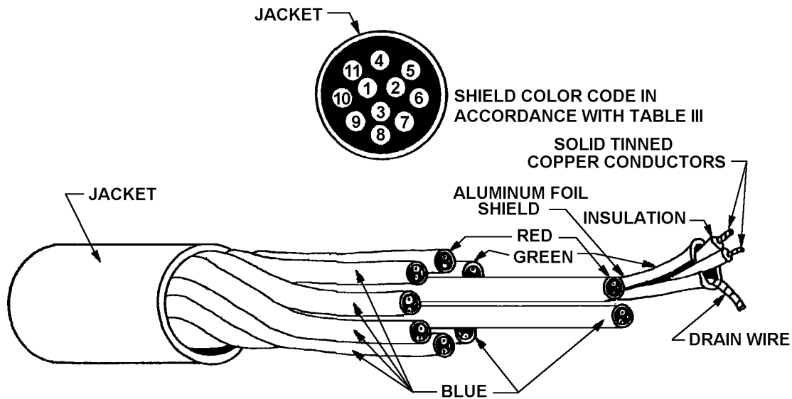
FIGURE 1. Cable illustration.
