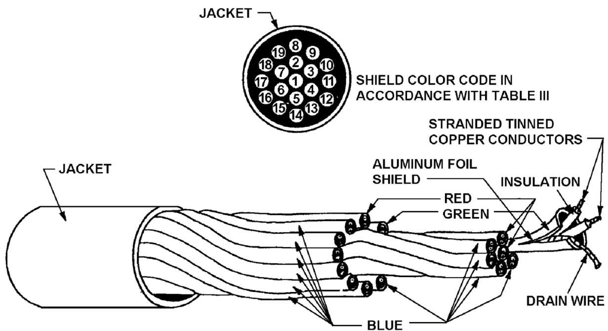
FIGURE 1. Cable illustration.
