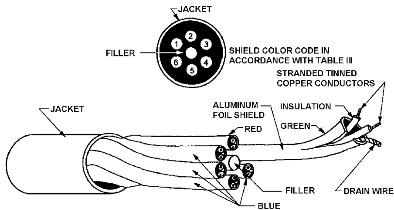
FIGURE 1. Cable illustration.
