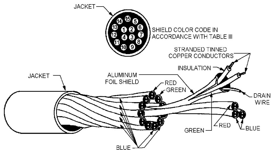
FIGURE 1. Cable illustration.
