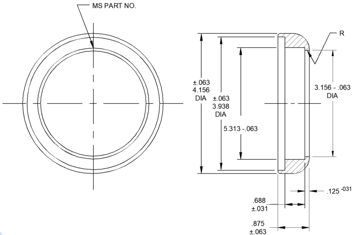
FIGURE 1. Dust cover. Part number: MS27272-1.
