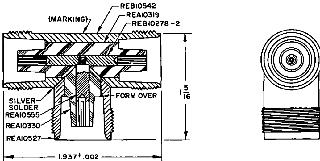
FIGURE 1. Type UG-413/U connector adapter.
