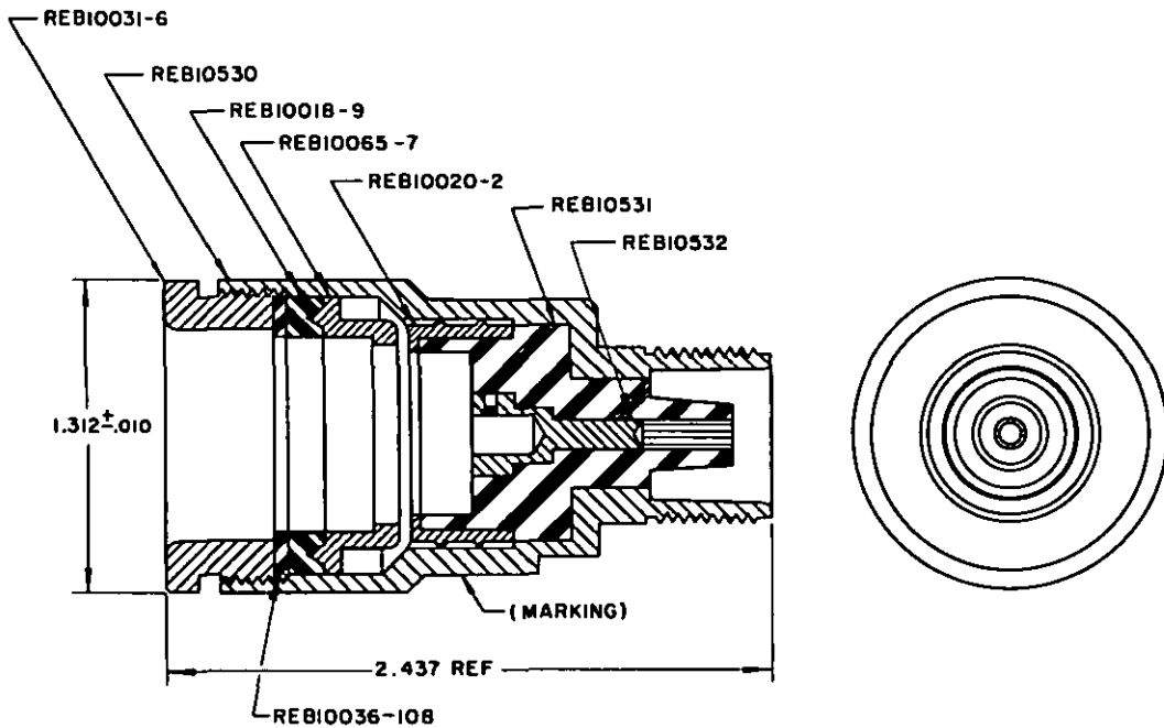
FIGURE 1. Type UG-333C/U electrical plug connector.
