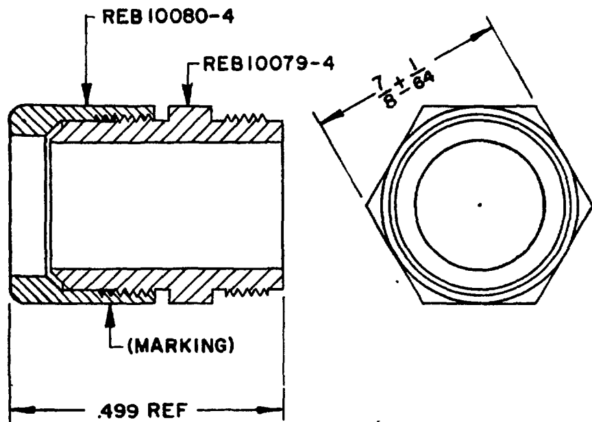
FIGURE 1. Type MX-1462/U armor clamp.
