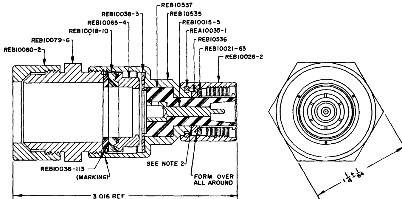
FIGURE 1. Type UG-926B/U electrical plug connector
