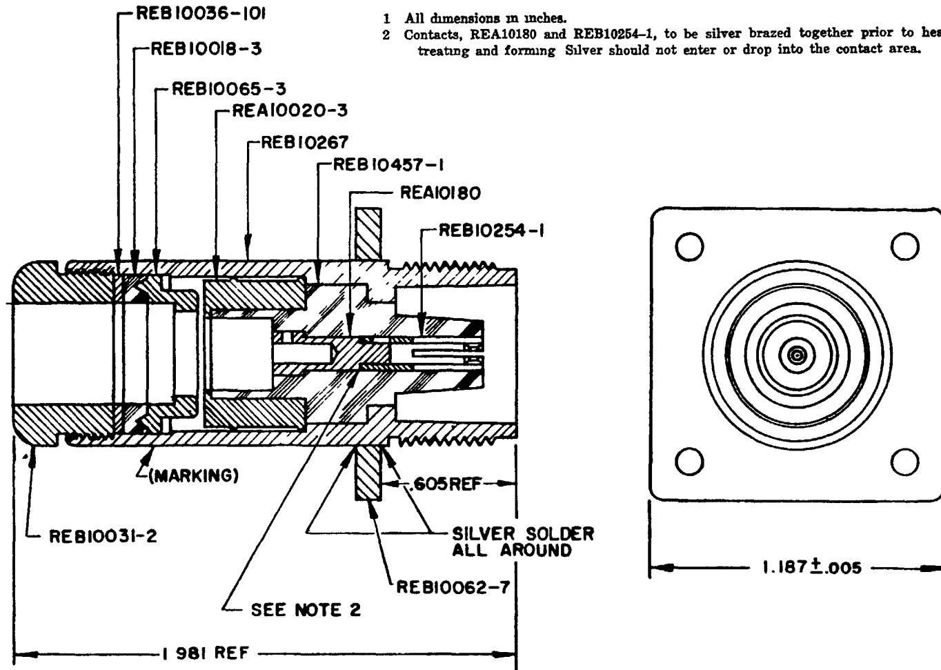
FIGURE 1 Type UG-427C/U electrical receptacle connector
