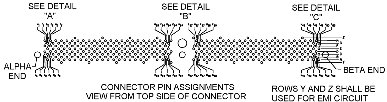
FIGURE 3. Printed wiring board layout - Continued.
