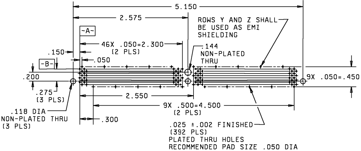
Printed circuit backplane grid layout (Connector side)
