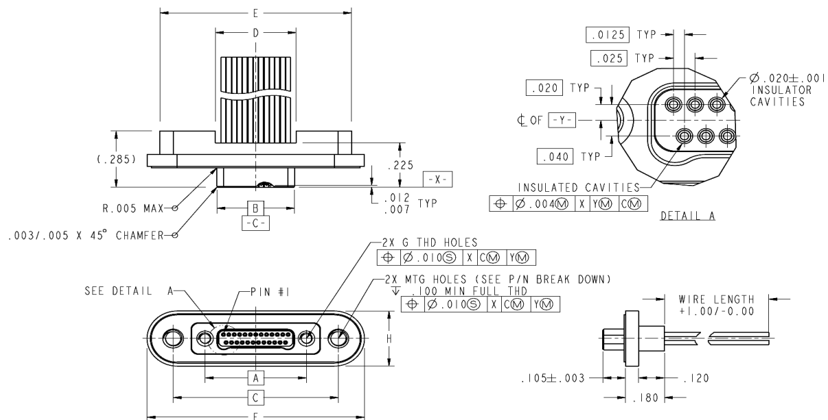
FIGURE 1. Plug, Rear Panel Mount dimensions and configurations.
