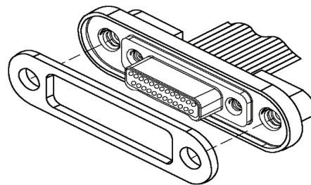
FIGURE 1. Plug, Rear Panel Mount dimensions and configurations.
