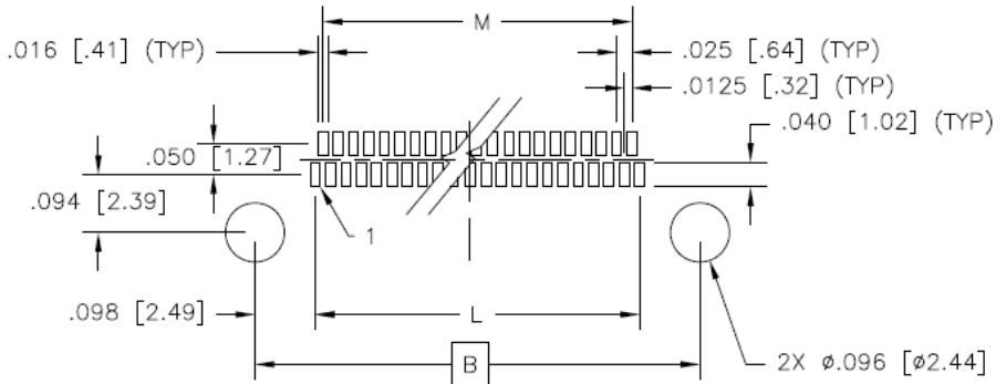
RECOMMENDED PC BOARD LAYOUT FOR SIZE 85 (COMPONENT SIDE)
