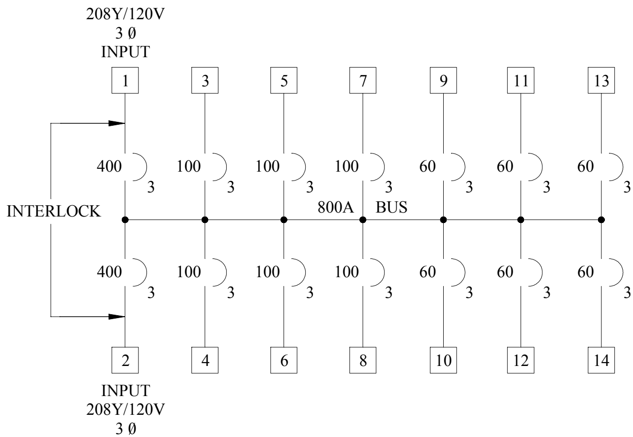
FIGURE 1. Single-line wiring diagram.
