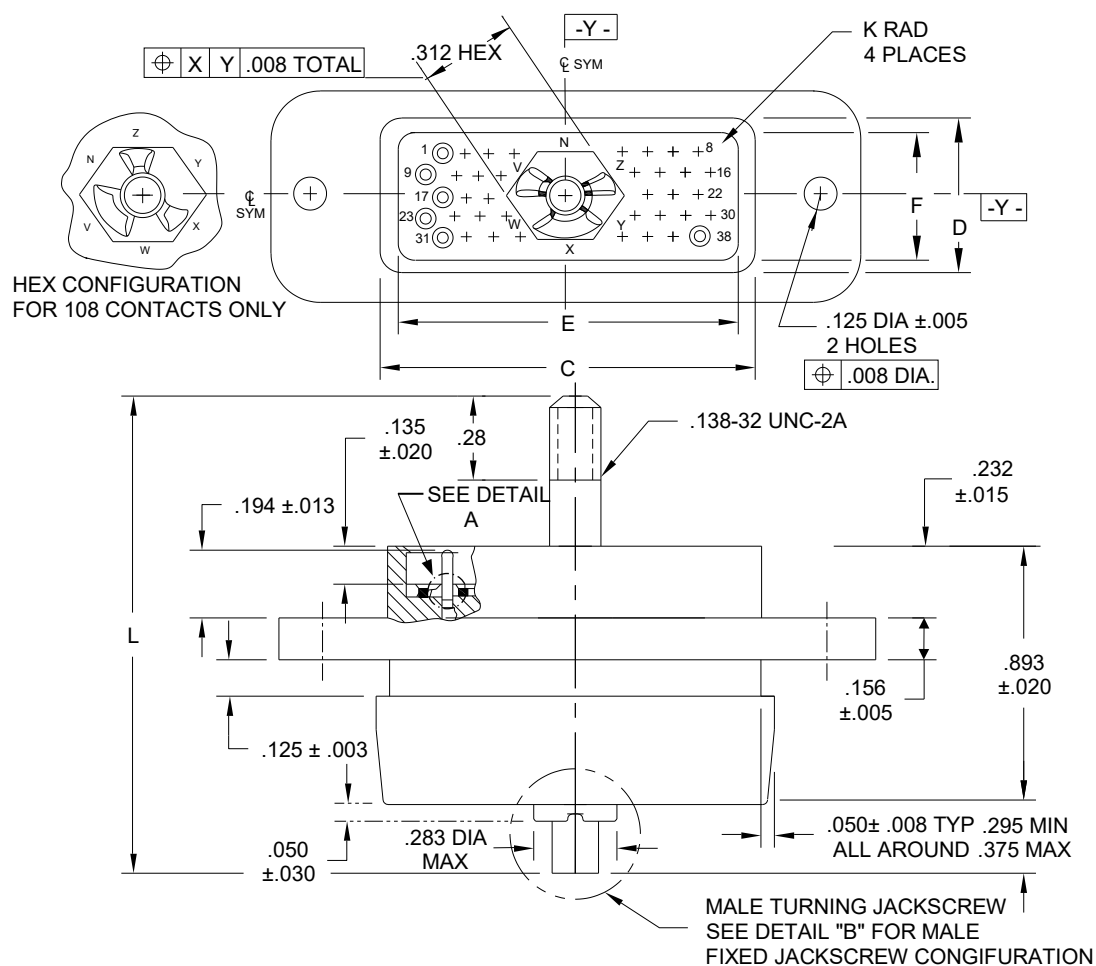
FIGURE 1. Connector, crimp removable pin contacts, class E.
