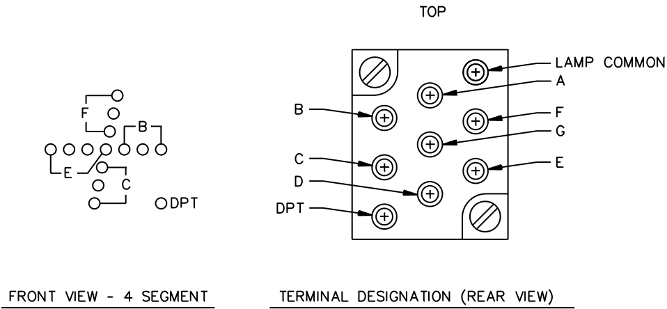
FIGURE 6. Truth table letter assignments for four segment sign display with decimal point.
