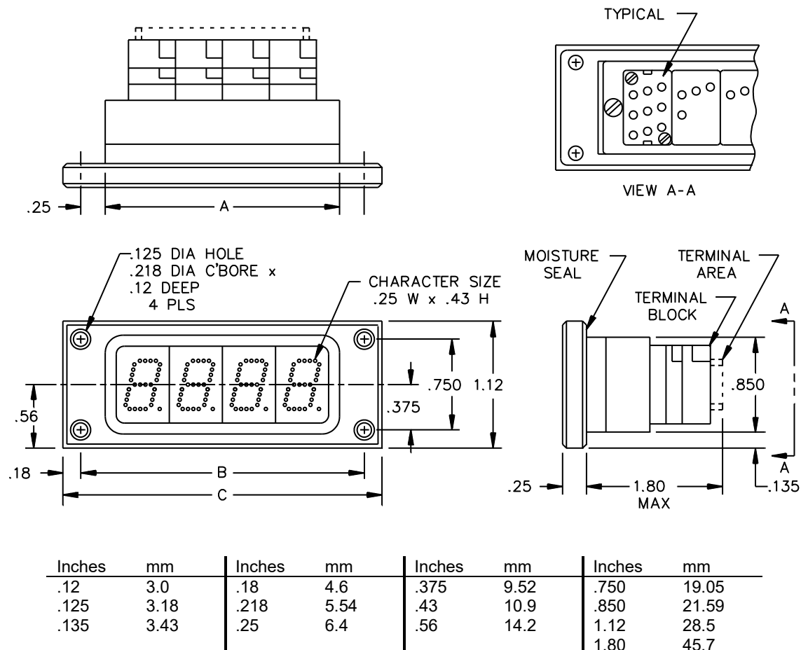
FIGURE 1. Type R02 display.
