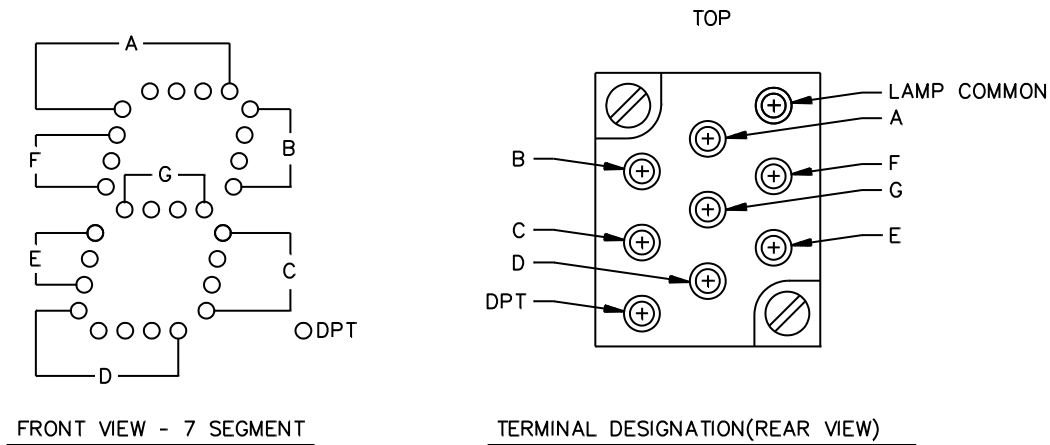
FIGURE 5. Truth table letter assignments for seven segment alpha-numeric display with decimal point.
