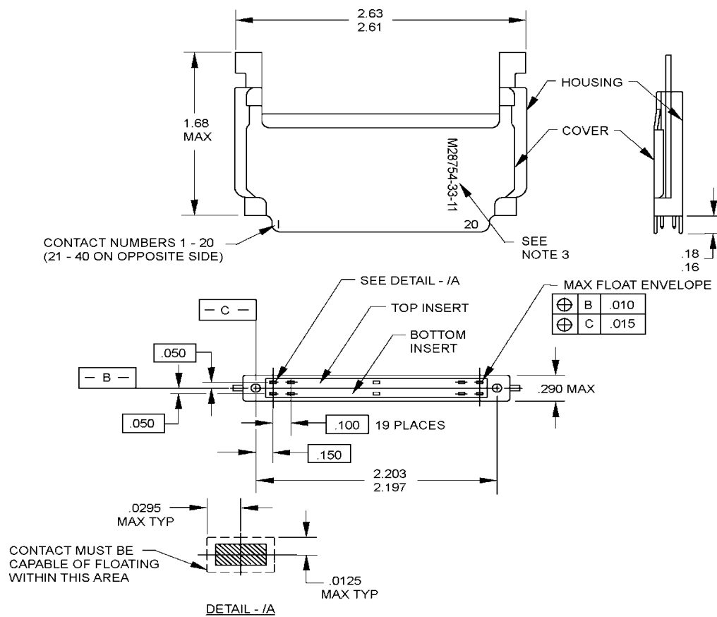
FIGURE 1. Connector assembly.
