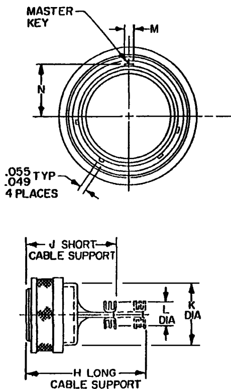
FIGURE 1. Plug dimensions.
