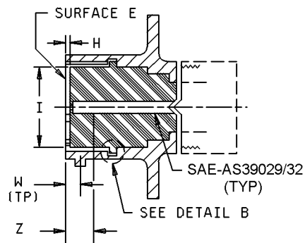
STYLE S (SOCKET INSERT)
