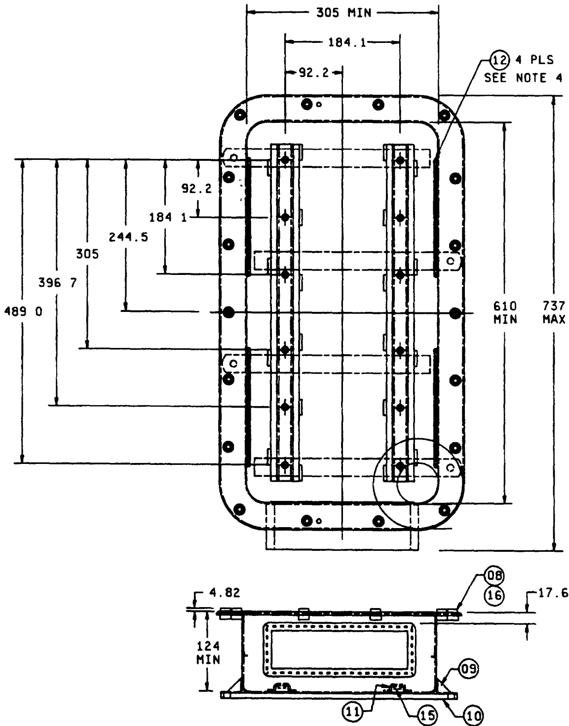
FIGURE 3 Box assembly
