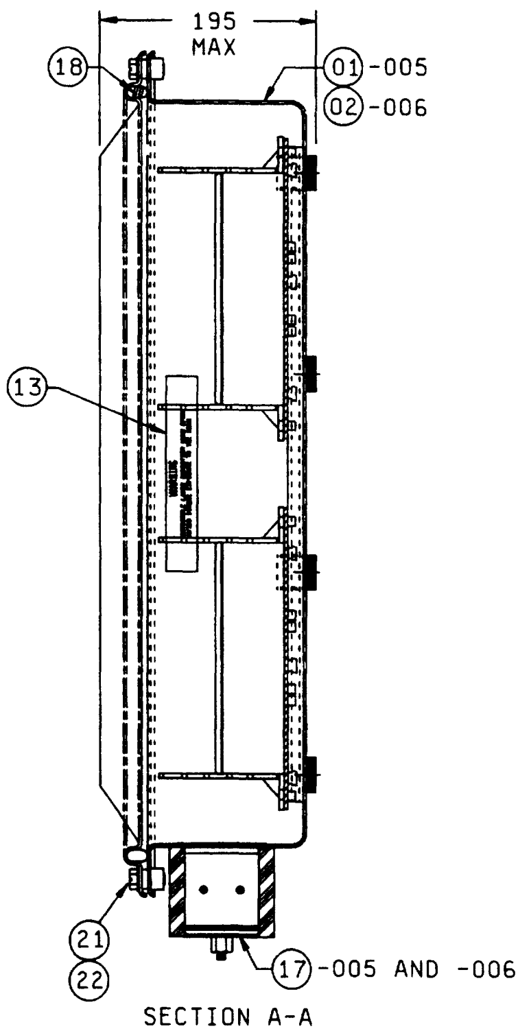
FIGURE 1 Enclosure assembly, M24728/2-005 and M24728/2-006 - Continued
