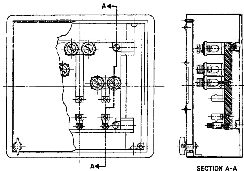
FIGURE 1. Fuse box assembly, typical. Item No. 01, 02 (Symbol 680 shown)
