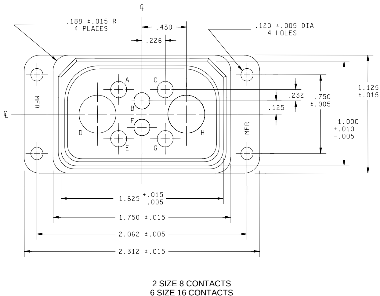
FIGURE 1. Type J, class M inserts containing pin contacts.
