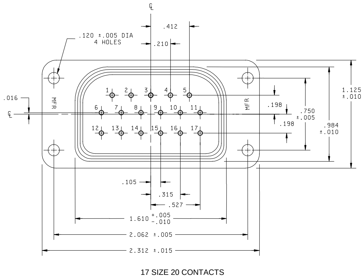
FIGURE 1. Type P, class F inserts containing socket contacts.
