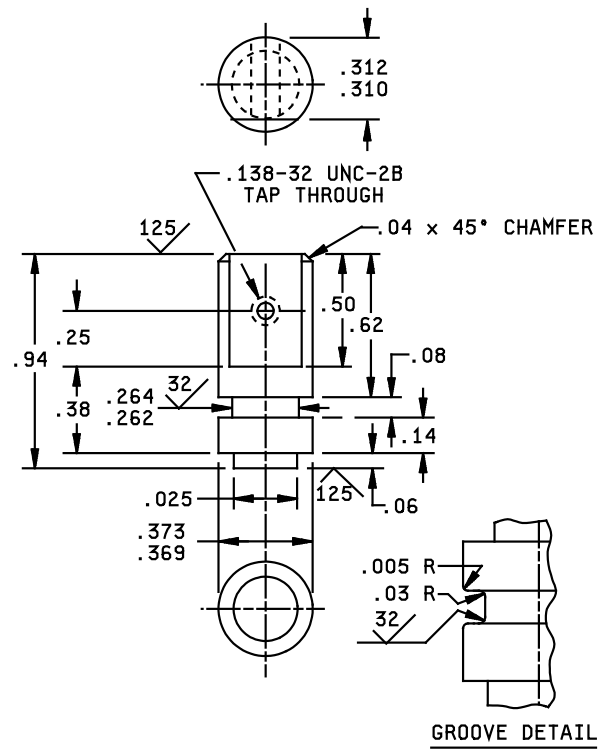
FIGURE 8. Shaft. (12)
