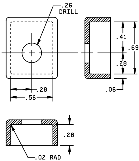
FIGURE 9. Coupler. (13)
