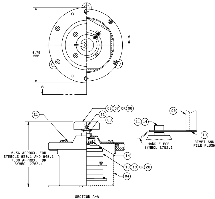
FIGURE 1. Switch, enclosed (typical). 01, 02, 03 (-001 shown)
