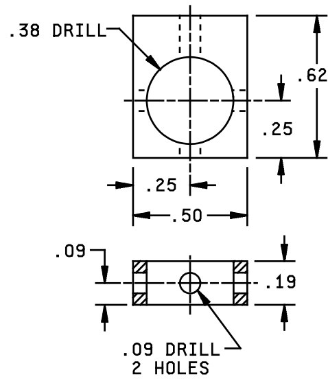
FIGURE 10. Coupler plate. 14
