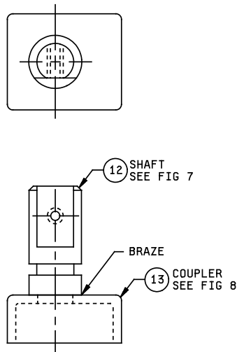
FIGURE 7. Shaft assembly. ⑪, ⑫, ⑬
