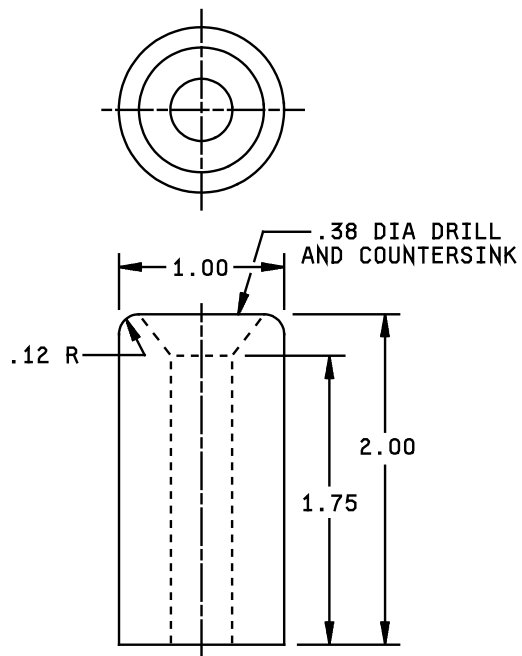
FIGURE 5. Handle knob. ⑨
