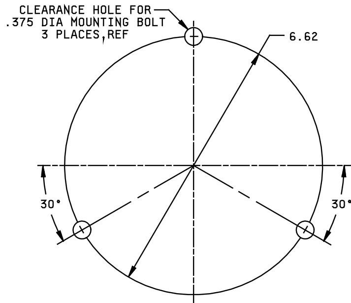
FIGURE 11. Mounting dimensions, ref.
