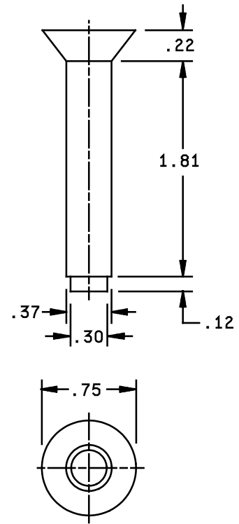
FIGURE 6. Knob pin. ⑩
