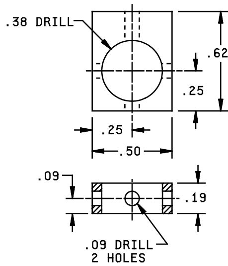
FIGURE 8. Coupler plate. (10)
