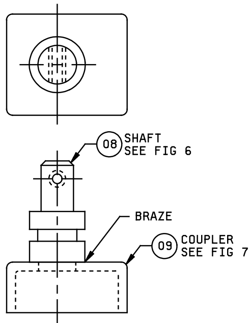
FIGURE 5. Shaft assembly. 07
