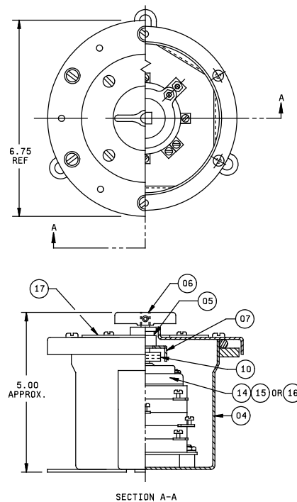
FIGURE 1. Switch, enclosed (typical). 01 02 03
