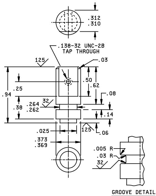
FIGURE 6. Shaft. 08
